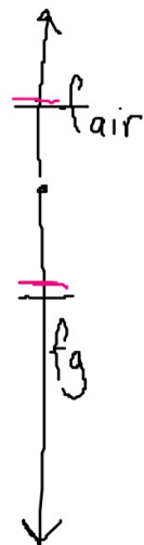
LM-12. Rock is falling at constant (terminal) velocity.
