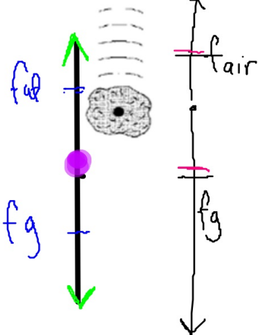
LM-12. Rock is falling at constant (terminal) velocity.
