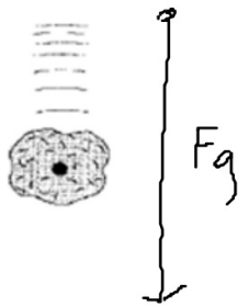
LM-10. Rock is falling. No friction.
